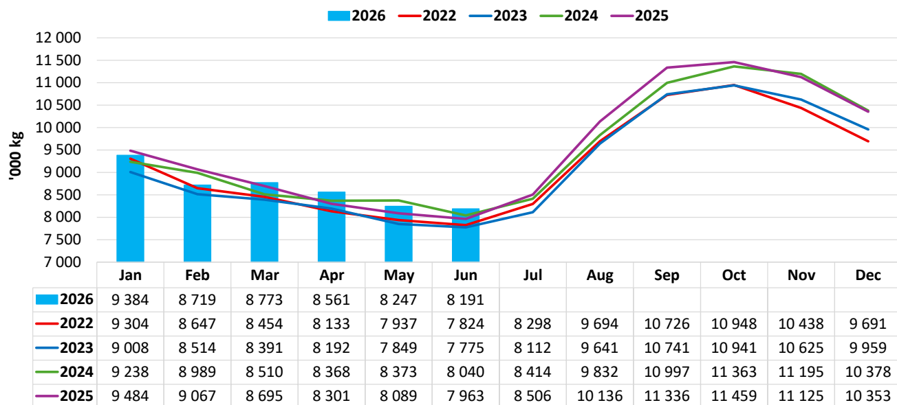
FIGURE 3: Monthly cumulative net imports, milk equivalent, January 2022 to May 2026.
