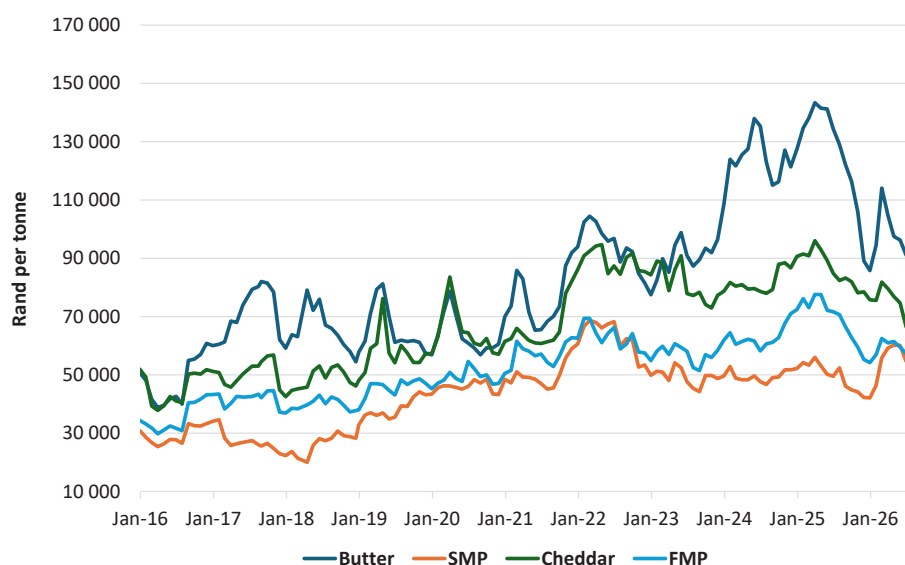
FIGURE 1: International dairy product prices (free on board), January 2016 to July 2026.
