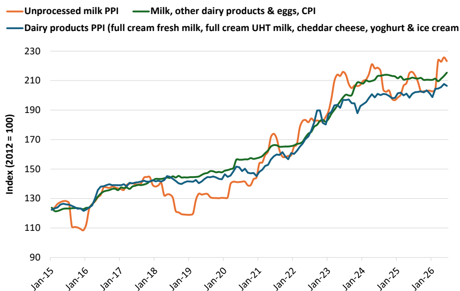
FIGURE 4: PPI indices of unprocessed milk and dairy products, and the CPI of milk, cheese, and eggs, January 2015 to June 2026.
