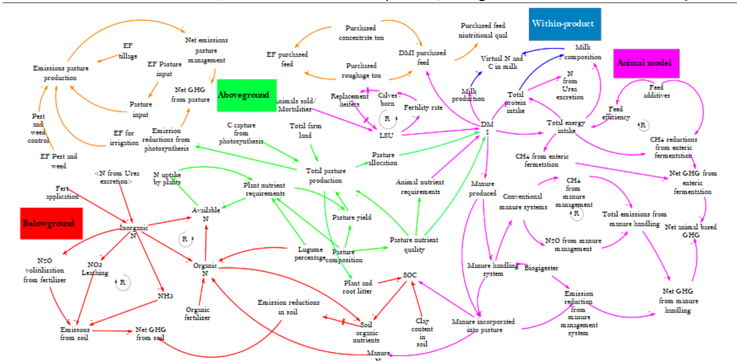
Figure 1: Causal loop diagram showing the flow of sources and sinks within a dairy farm system. [Note: Red sub-model: belowground; Green sub-model: aboveground; Purple sub-model: animal model; Blue sub-model: within-product; Orange sub-model: external sources].
